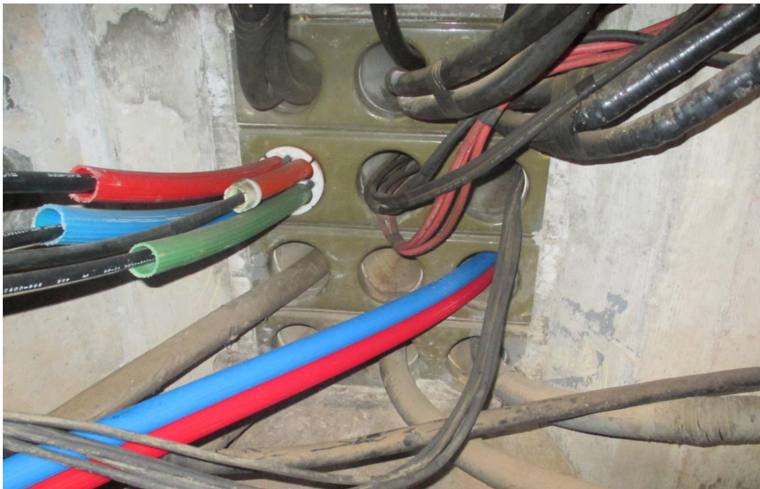
Figure 4.7 KUB Network with Innerduct and Cable
