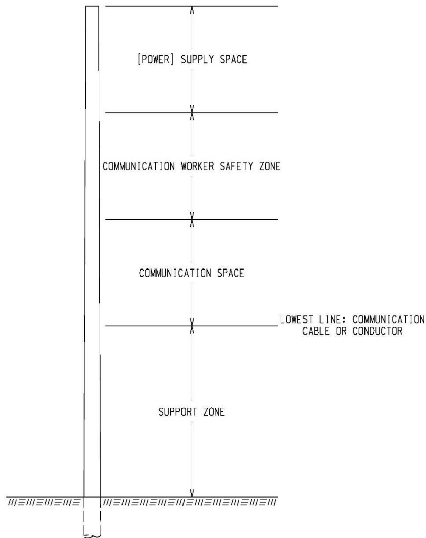
Figure 3.4 Work Zones on KUB Poles
